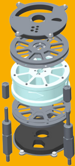
Rubber sealing plate set for 2.5, 6 and 12 liters
