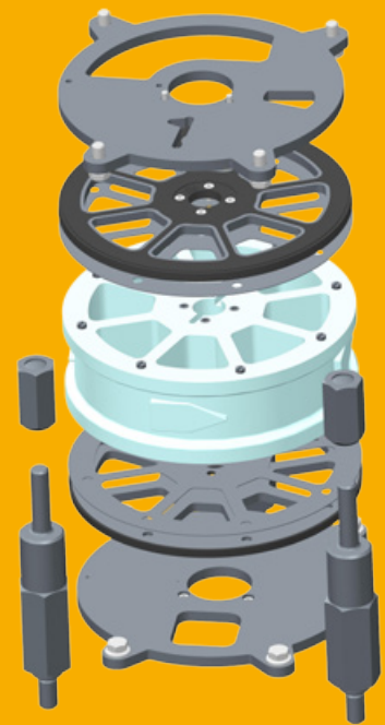
Rubber sealing plate set for 2.5, 6 and 12 liters
